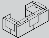
TRA129 3354 / 1705 / 1159 132" / 67 1/8" / 45 5/8" TRA130 3754 / 1705 / 1159 147 3/4" / 67 1/8" / 45 5/8" TRA131 4154 / 1705 / 1159 163 1/2" / 67 1/8" / 45 5/8" TRA132 4554 / 1705 / 1159 179 1/4" / 67 1/8" / 45 5/8"
